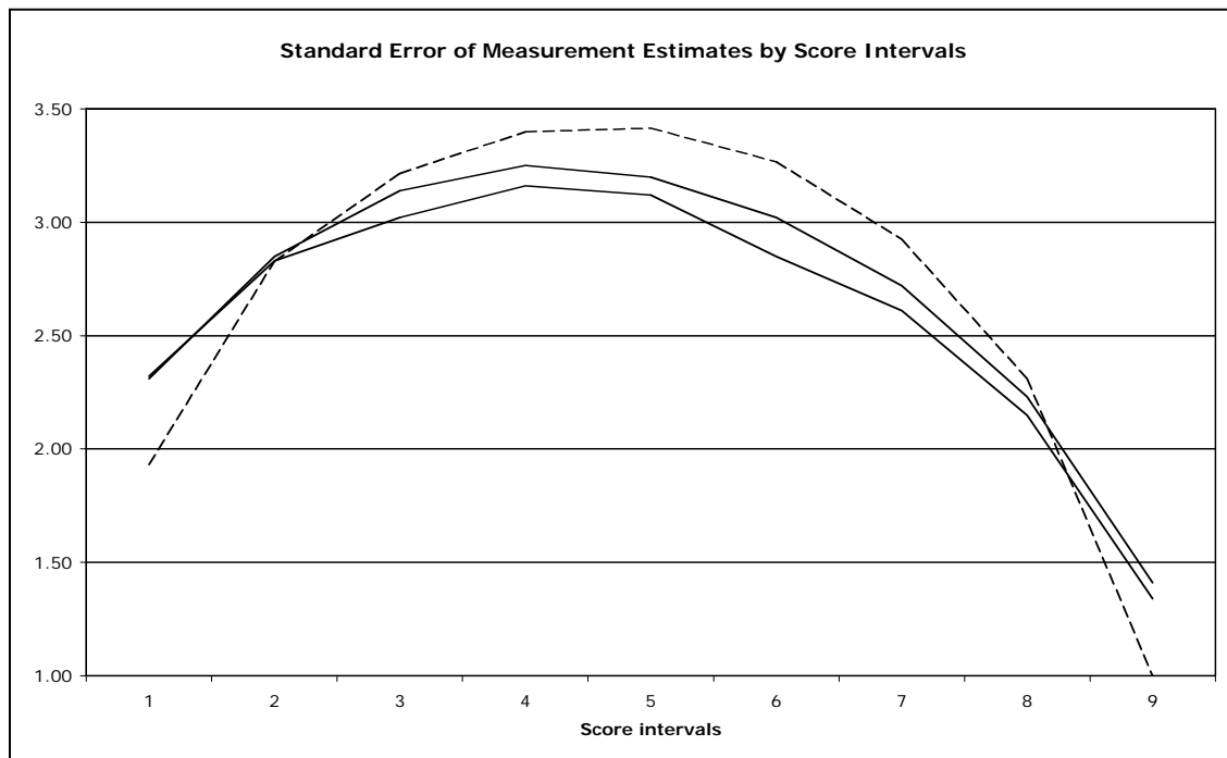
Figure 2: Feldt data with n = 15,546
