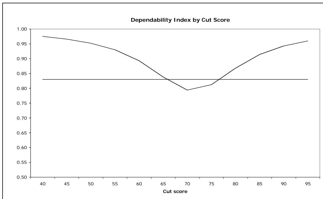
Figure 5: Dependability index, \Phi(\lambda) , by cut score value
